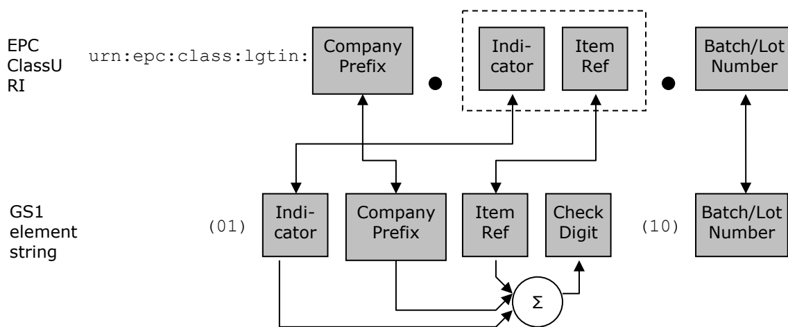
Figure 7-14 Correspondence between LGTIN EPC Class URI and GS1 element string
