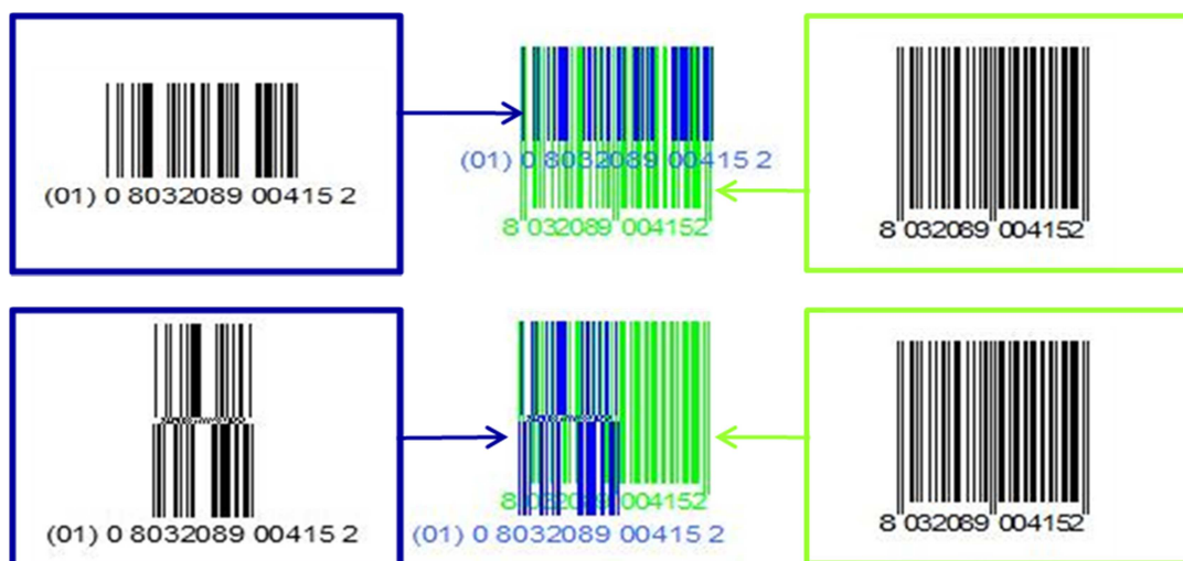
Figura 7-5: Confronto GS1 DataBar Omnidirectional e Omnidirectional Stacked con EAN-13
