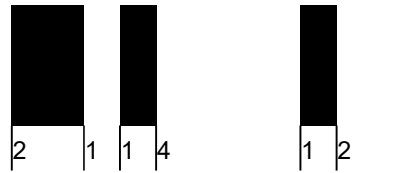
Figure 5.4.3.1-2 illustrates the encoding of one the symbol character value 35 , which represents the single data character C in both code sets A or B or the two distinct data character digits 3 and 5
