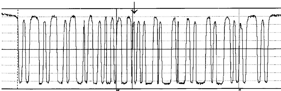
Figura 5.12.5.12-2 Scan Reflectance Profile of symbol with low decodability character
