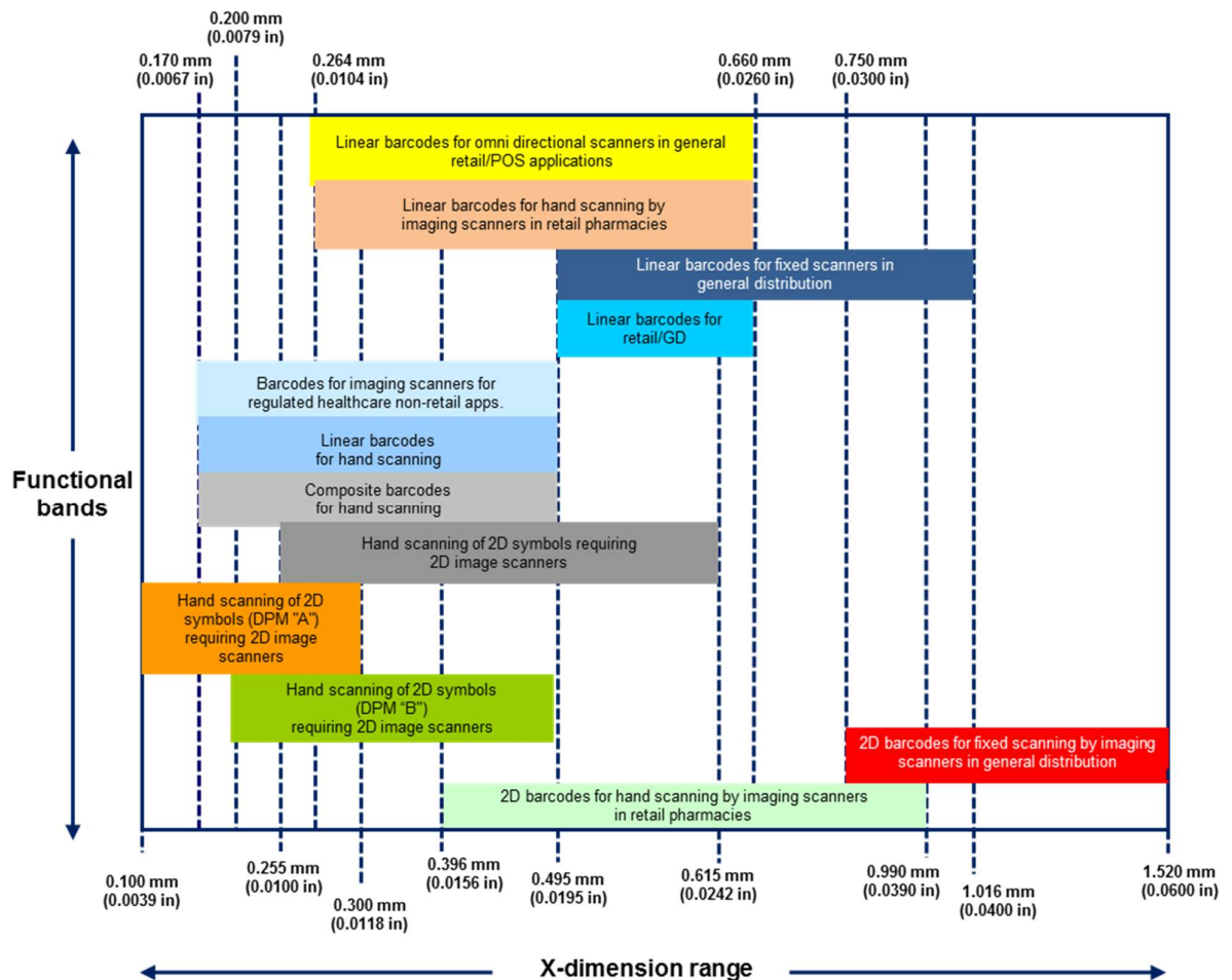
Figure 5.12.2-1 GS1 scanner functional operative bands
