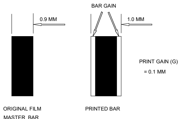
Figura 5.12.4.2.1-1. Example of bar width adjustment
